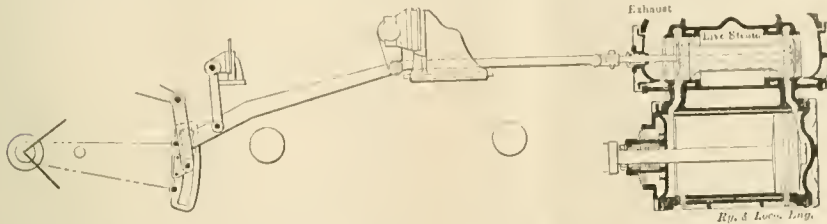
EXAMPLE OF DIRECT MOTION, INSIDE ADMISSION PISTON VALVE.
